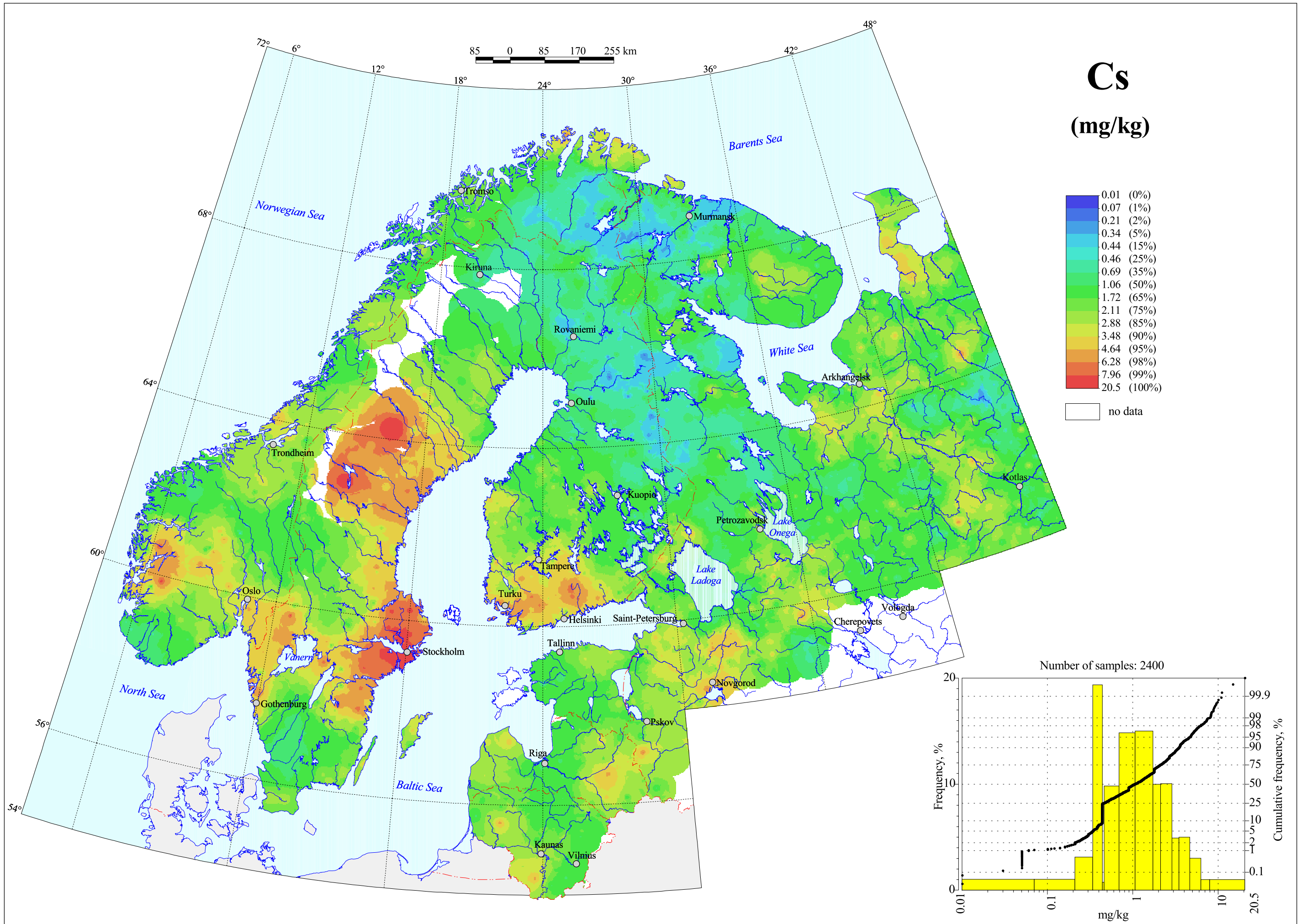
Cesium in C-horizon, Grain Size <2 mm, Total Content
